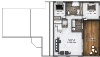
DWELLING 2 UPPER FLOOR PLAN
