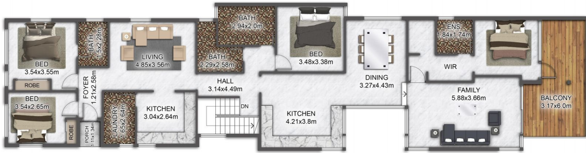
LEVEL 2 FLOOR PLAN
