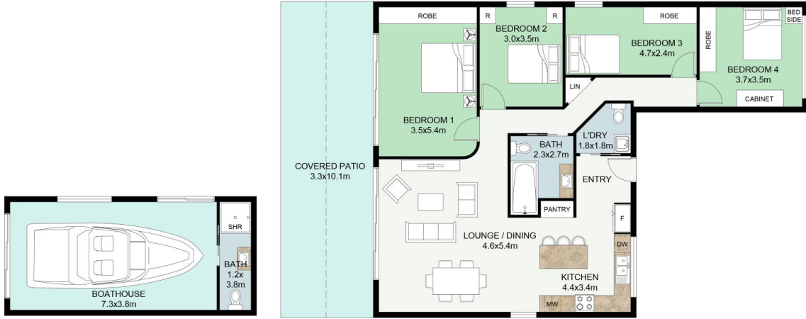
FLOOR PLAN
